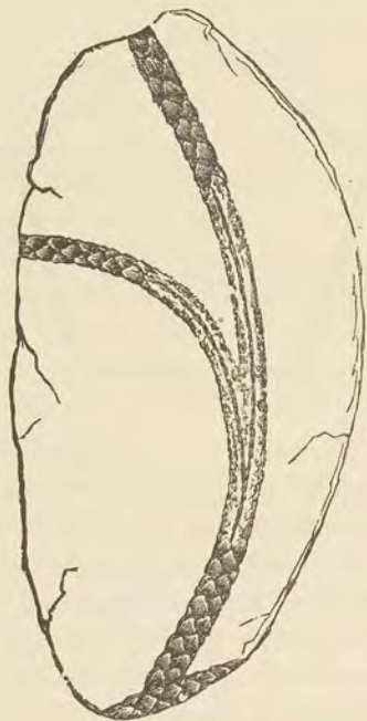
IMBRICATED STEM. ( Helmsdale. )
